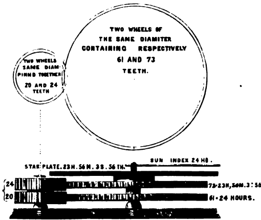
Section of the Wheel-work of Ferguson's Solar and Sidereal Clock.
